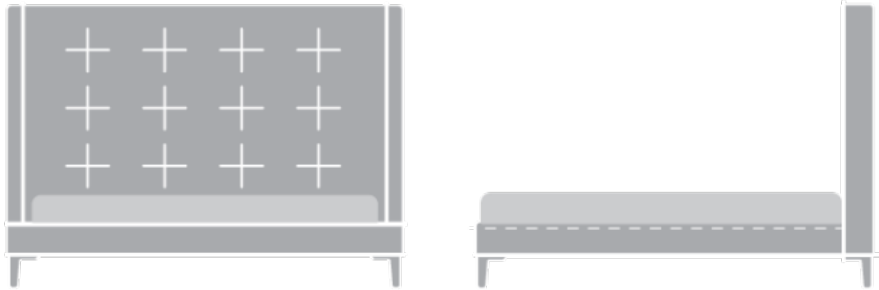
B120-20K60HT 83"W x 90"D x 60"H; 13½"SH
